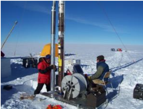
Ice Coring
